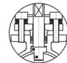
The disc spring loaded packing pressing mechanism is adopted.
