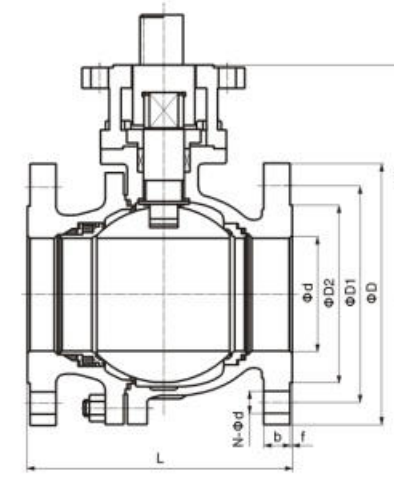
Floating cast steel ball valve
