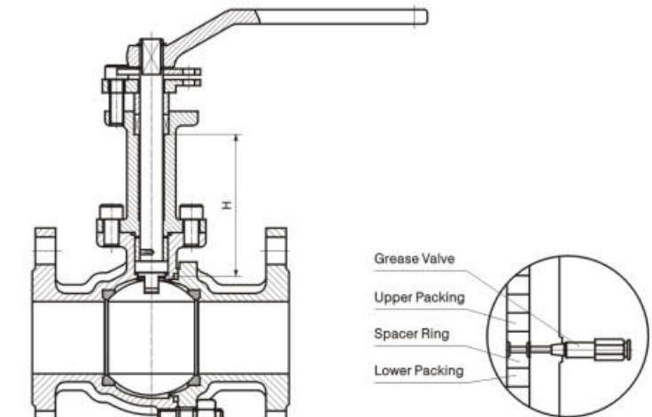
Double packing combination chart
